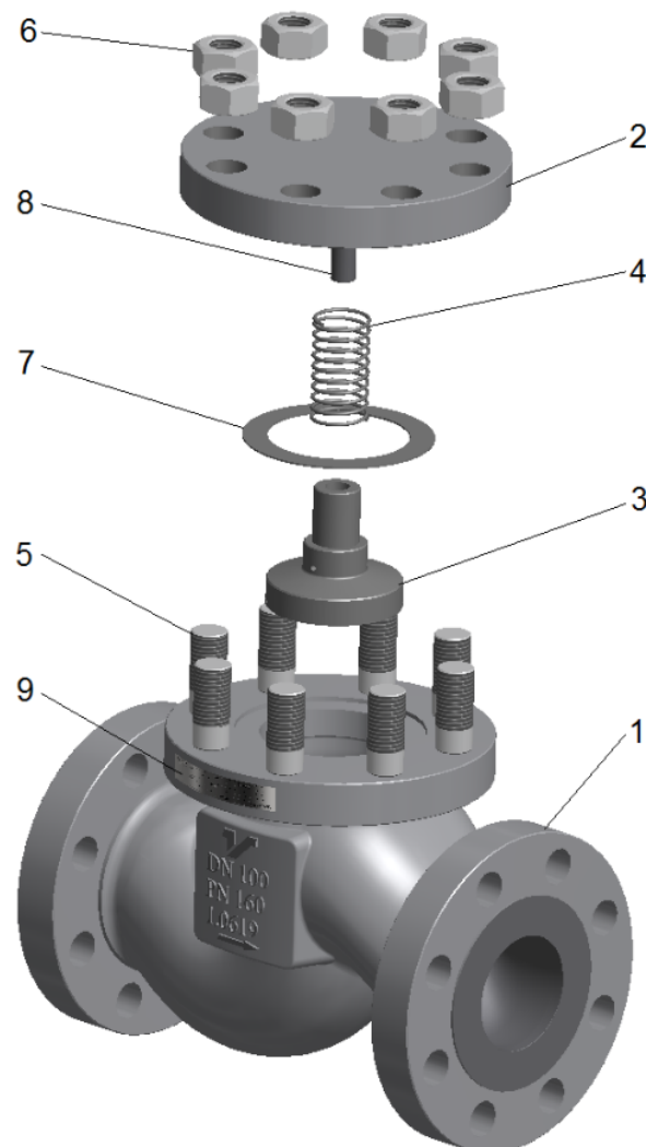
Fig. 1 Parts
