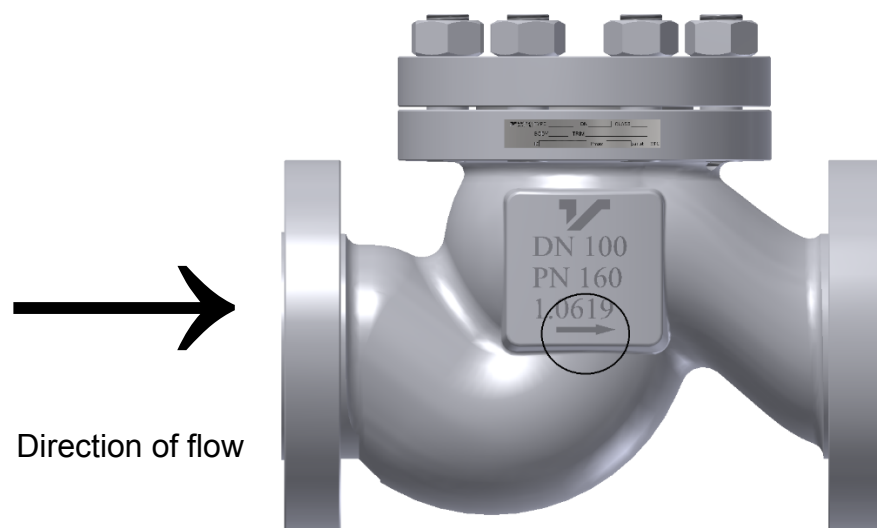
Fig. 2 Allowed mounting position
