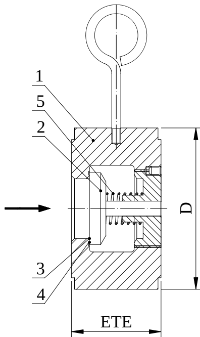
Drawing B.8.1 Parts and dimensions
