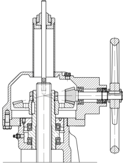
Gear operated
