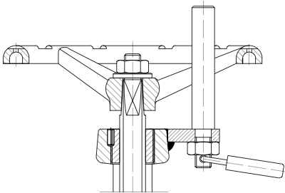
Locking device
