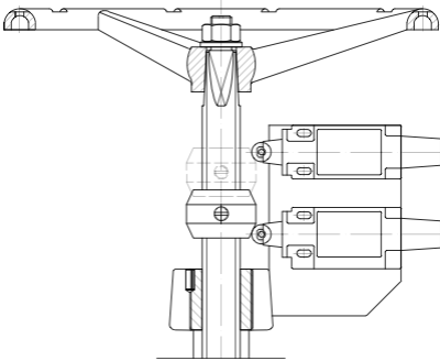
Limit switches
