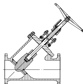
Regulacioni ventil Y-Tip [VENRY]
